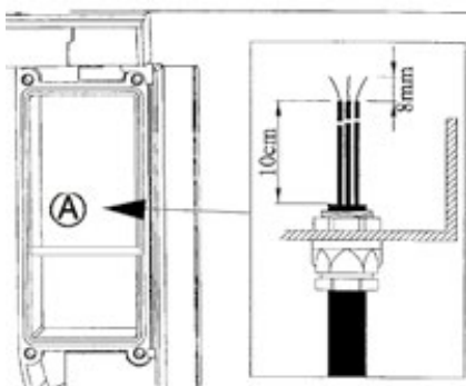
Connection box
